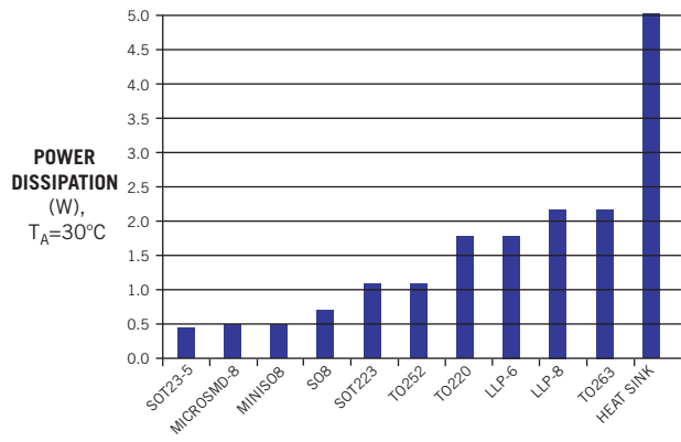
POWER-DISSIPATION CAPABILITIES OF COMMON PACKAGES ( T_A=30^\circ\text{C} )
