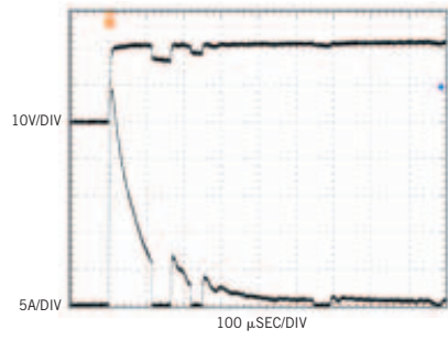
Figure 2 The mechanical relay, K_1 , by itself exhibits contact bounce on closure as shown.
