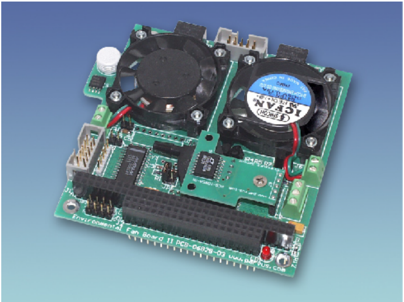
The ThermoCool Environmental Fan Card II offers temperature-controlled cooling plus humidity and pressure monitoring for PC/104 systems.
