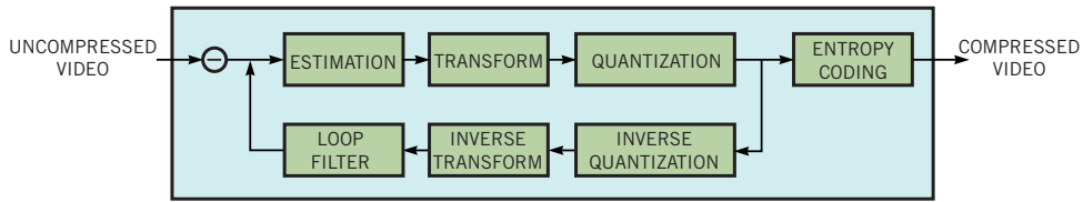
Figure 1 H.264 computes the differences between actual incoming video and estimated/transformed video, using either motion estimation or intraframe estimation. So, only the video and the difference appear in the compressed-video stream.
