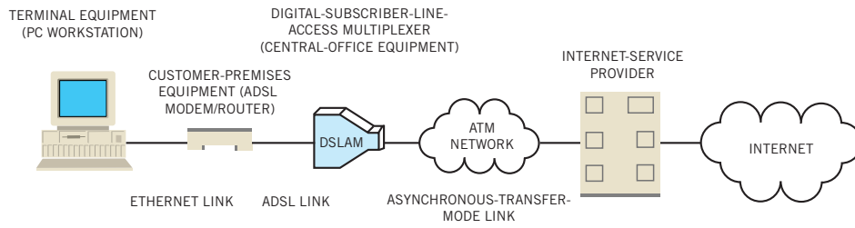
Figure 1 The PPPoA (point-to-point protocol over ATM) service mirrors a dial-up connection to bond USB/Ethernet traffic to an ATM environment via an ADSL link.
