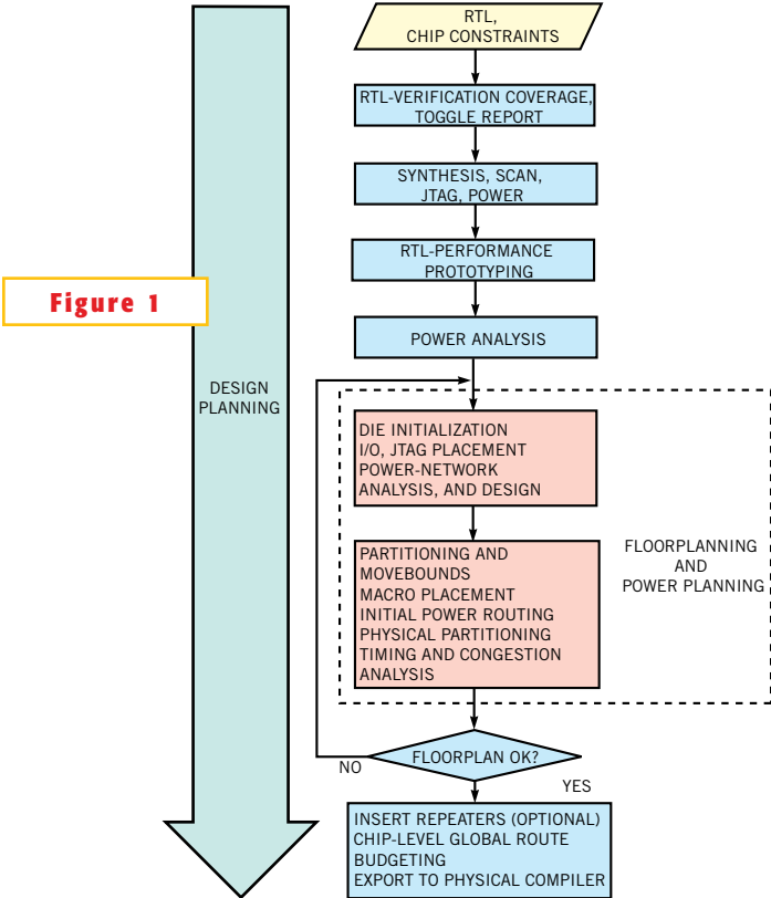
Design planning occurs in parallel with the stages of RTL maturity. Early floorplanning and power planning help guide RTL development and vice versa.
