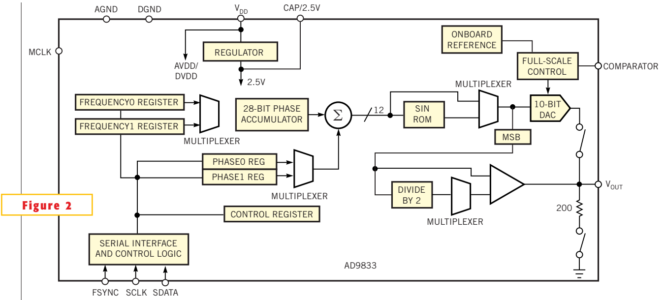
This DDS chip generates signals with 0.1-Hz resolution from a 25-MHz clock.
