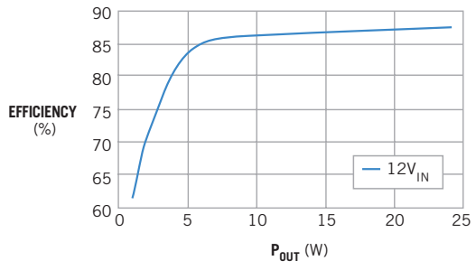
Figure 5 The conversion efficiency of the circuit in Figure 1 is well over 85%.
