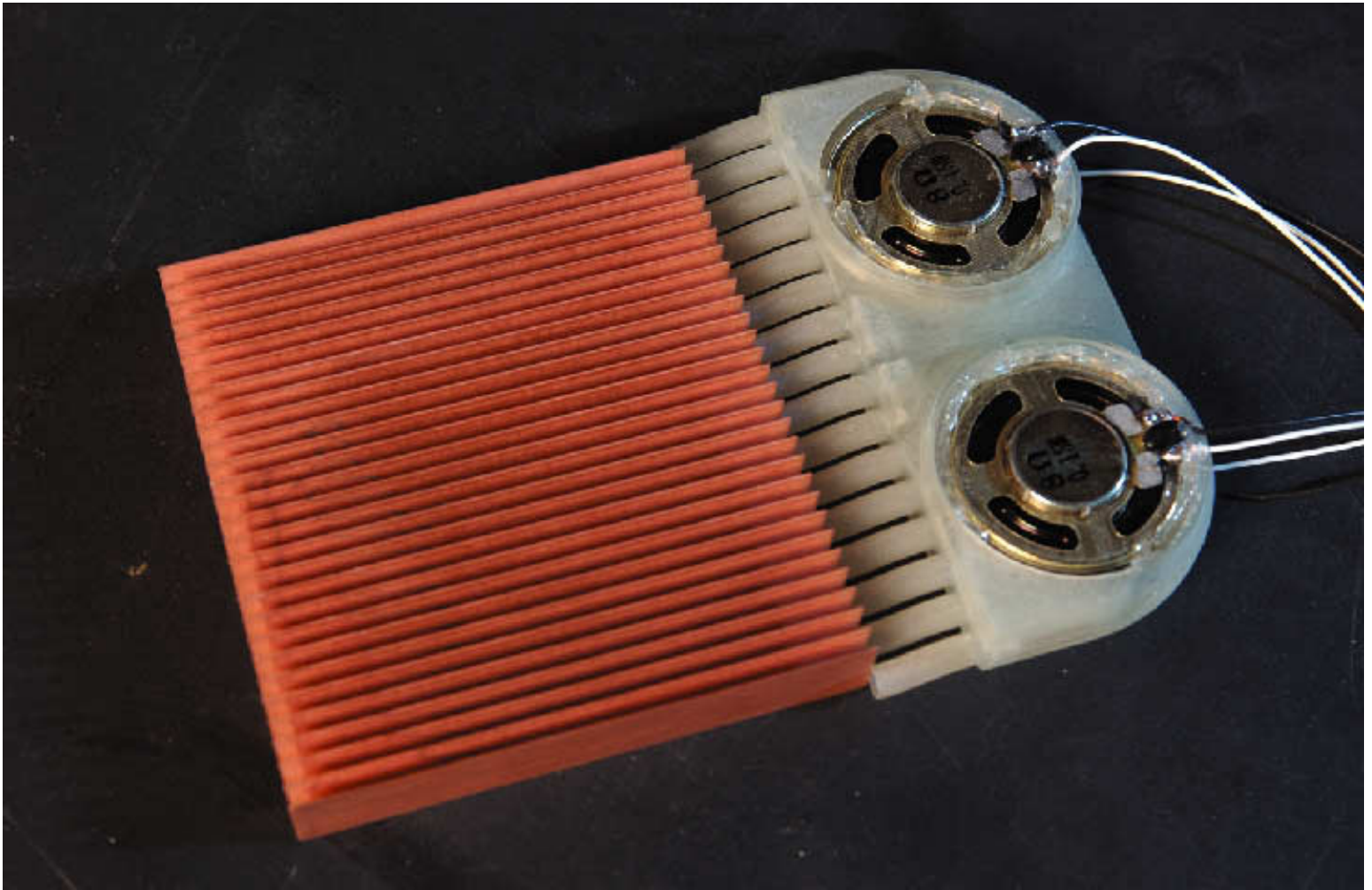
In a prototype SynJet, vibrating diaphragms (right) produce jets of turbulent air that flow out of tubes (white) and into the cooling fins of a component.
