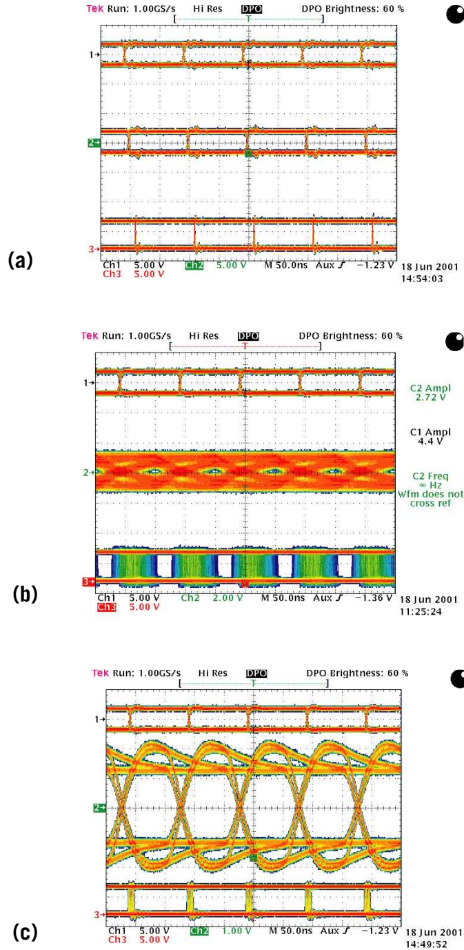
Eye patterns show cable compensation after 1m with no equalization (a), 300m with no equalization (b), and 300m with THS4140 equalization (c).
