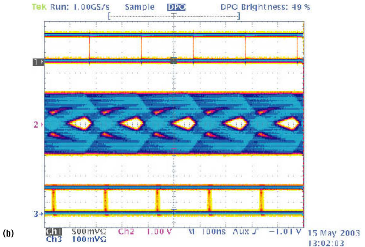
Oscilloscope patterns show RS-485 signaling through a 500m cable at 5 Mbps without receiver equalization (a) and with receiver equalization (b).
