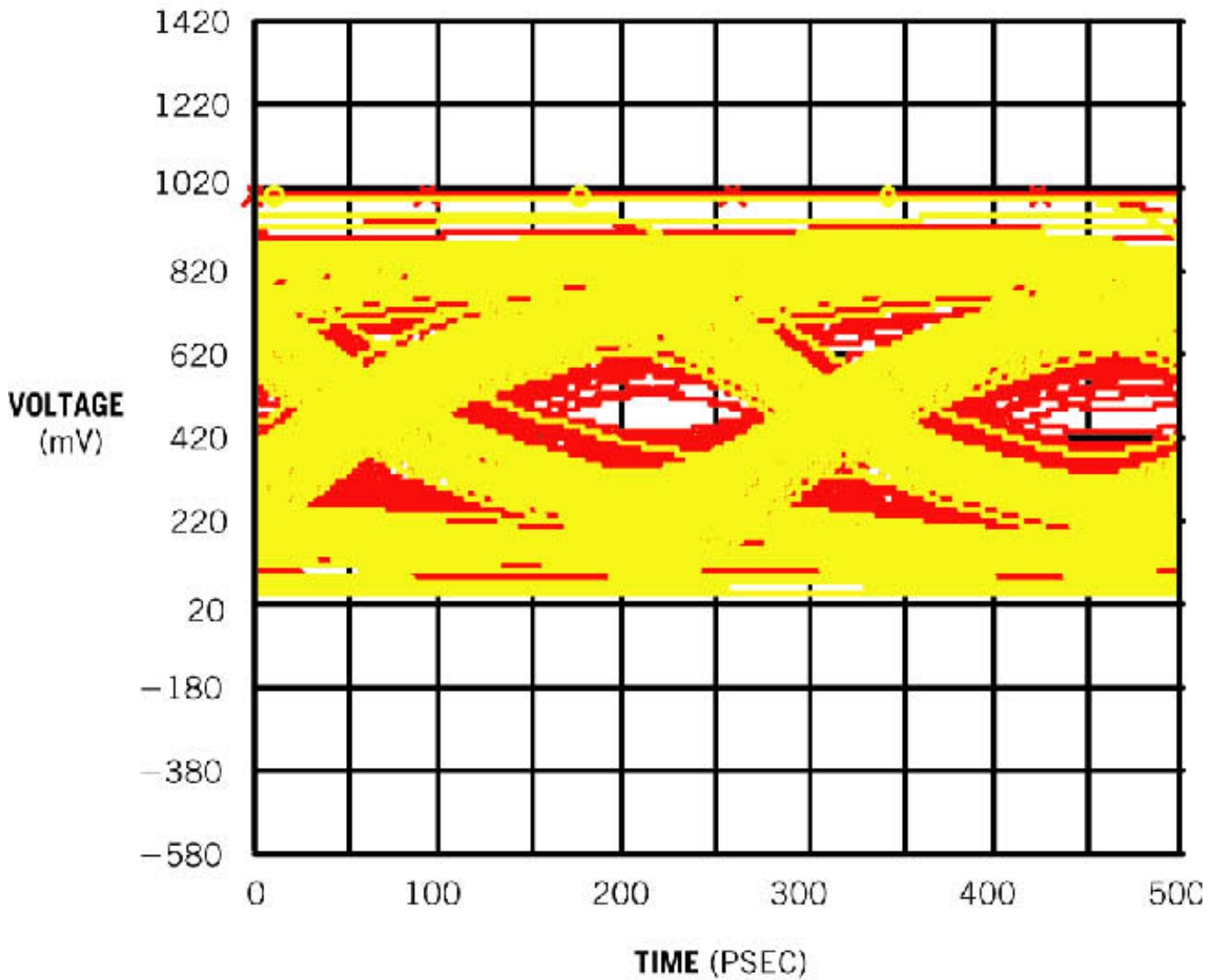
These eye diagrams show 2-Gbps signals that have traveled through 50Ω, 40-in. backplane traces with 0.004-in.- and 0.008-in.-wide lines in FR4 (simulated with Mentor Graphics' HyperLynx).
