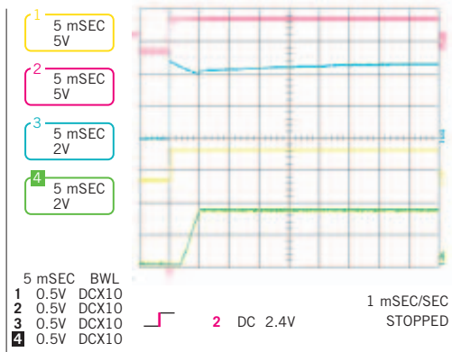
Figure 2 This circuit shows a normal start-up sequence for the circuit in Figure 1.
