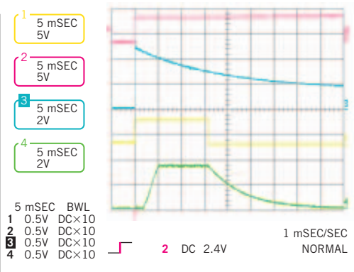
Figure 3 These traces represent start-up with the second output of a two-output regulator shorted.
