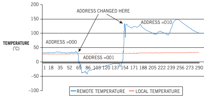
Figure 2 The ADT7461 measures the temperature of the selected sensor without interference from the other transistors with these results for ambient-, hot-, and cold-temperature measurements.
