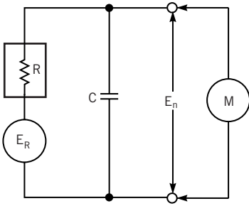
A resistor-noise model includes the parasitic shunt capacitance.
