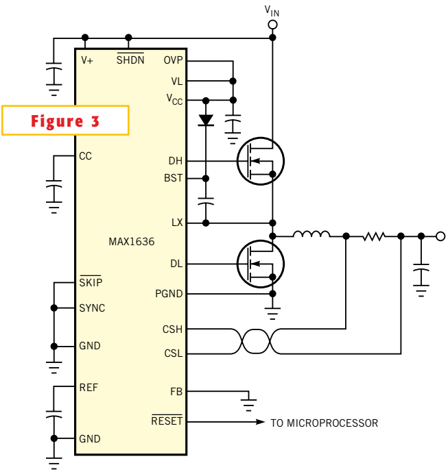
IC_1 in Figure 1 normally operates as a high-power buck converter.
