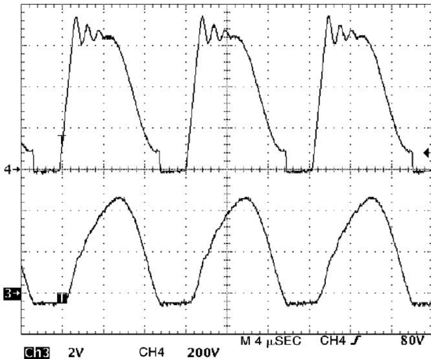
These waveforms illustrate the operation of Figure 1's circuit without the auxiliary winding.
