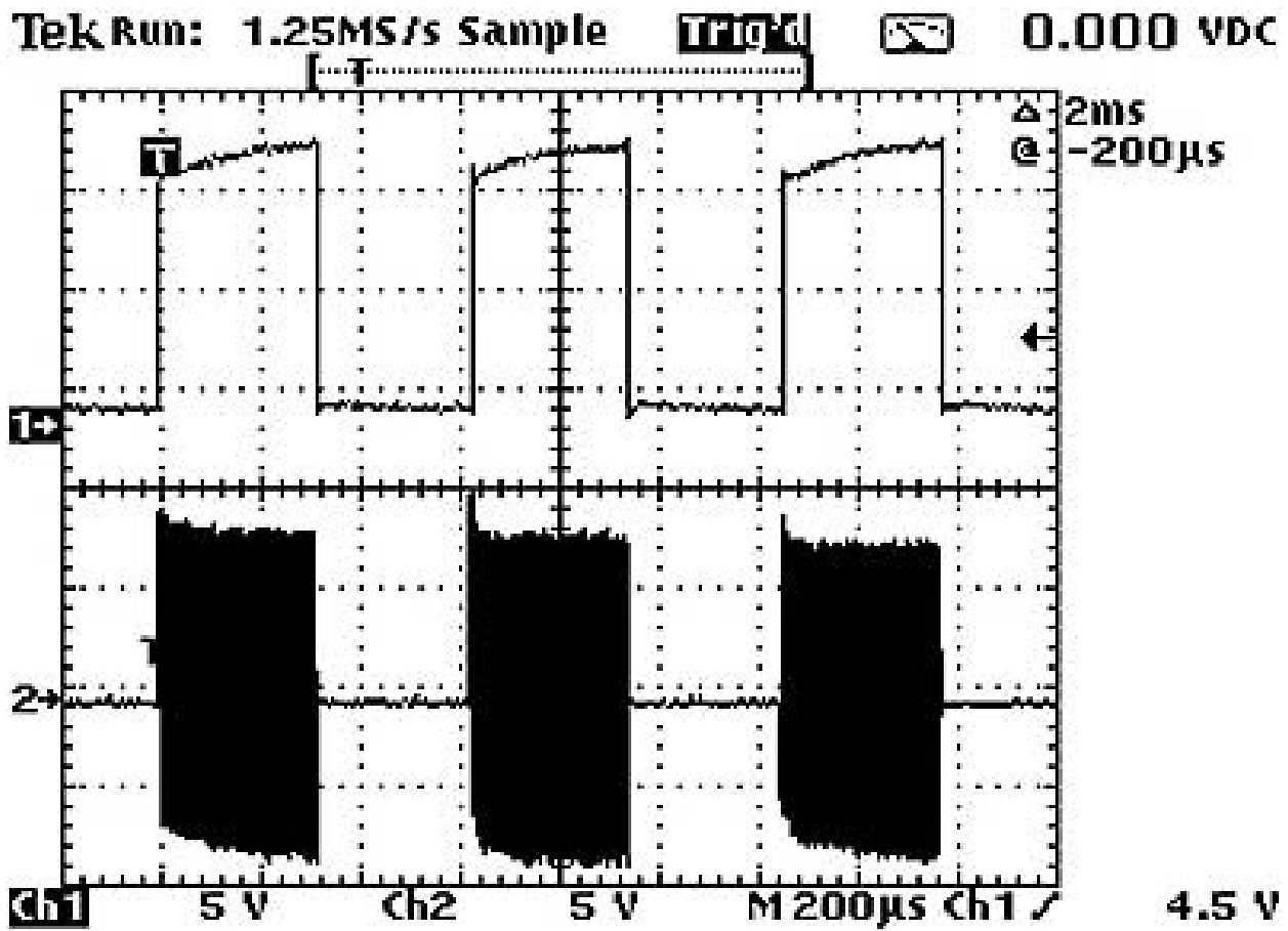
The top trace is the gate-drive voltage to the MOSFET; the bottom trace, the ac signal across the transformer secondary.
