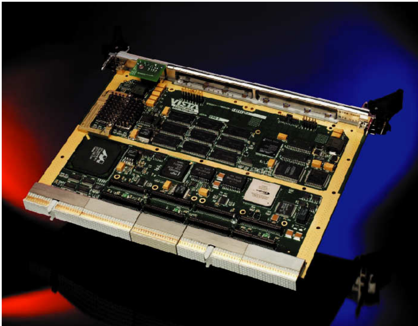
Vista Controls' PPC G4C single-board computer incorporates conduction cooling for an expanded operating-temperature range.
