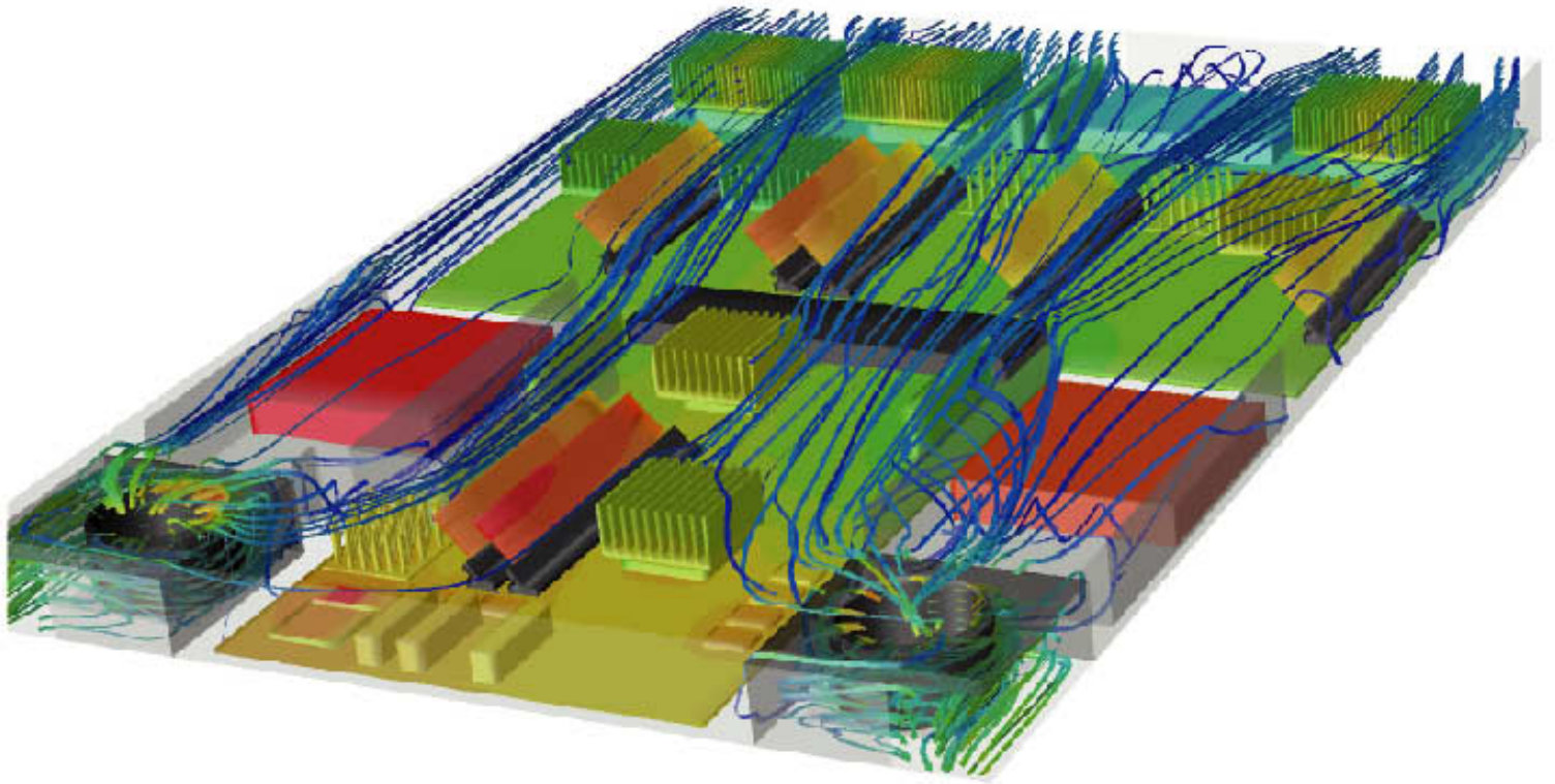
The thermal model of a 1U server using the Icepak analysis package shows colors representing surface temperatures and flow ribbons indicating airflow.
