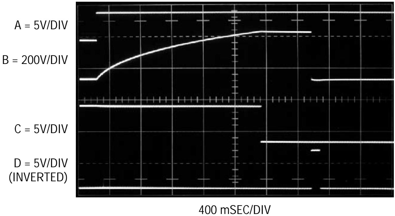
Capacitor-charging waveforms include charge input (Trace A), C_1 (Trace B), "done" output (Trace C), and "trigger" input (Trace D).
