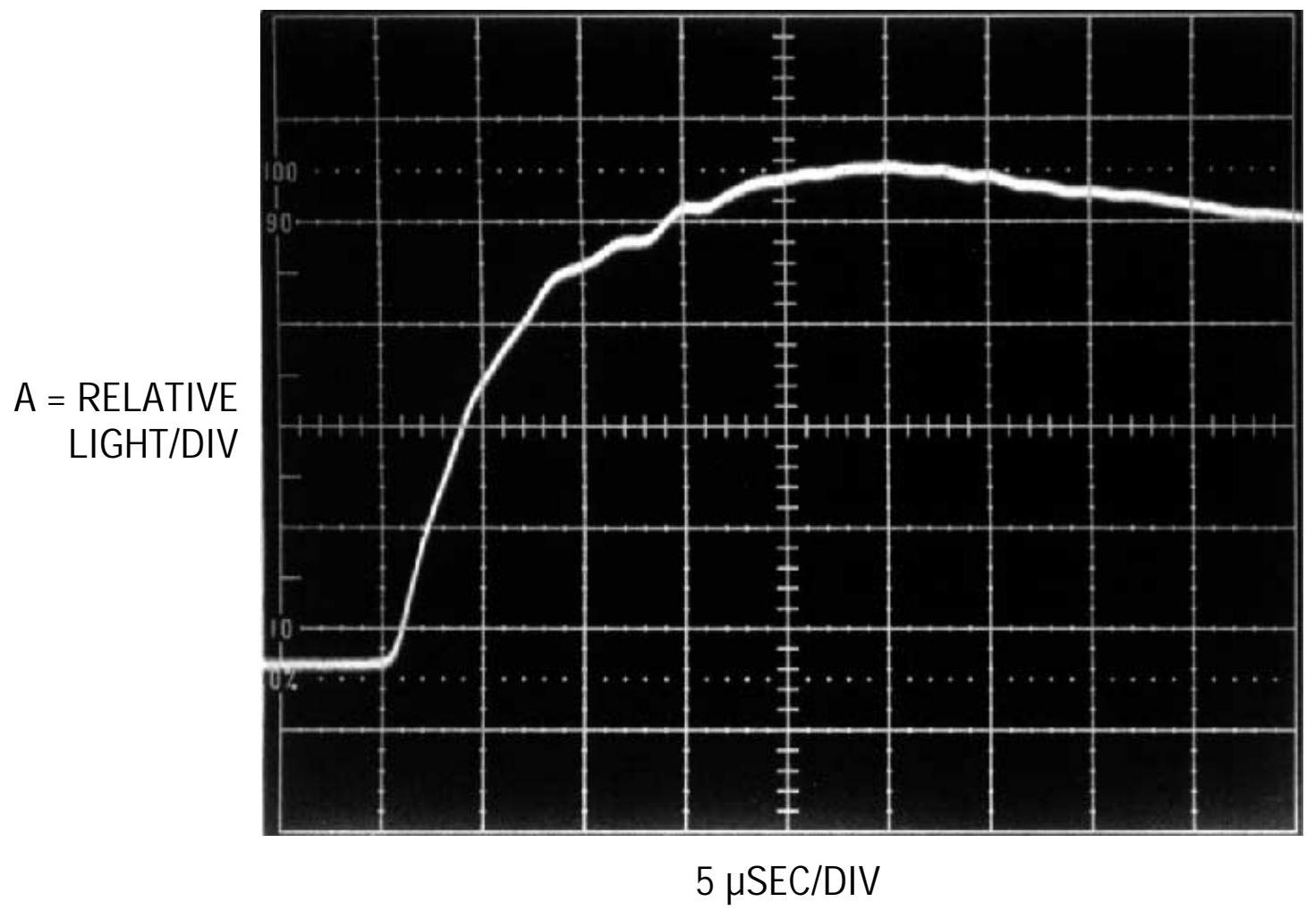
The smoothly ascending flash-lamp light output peaks in 25 msec.
