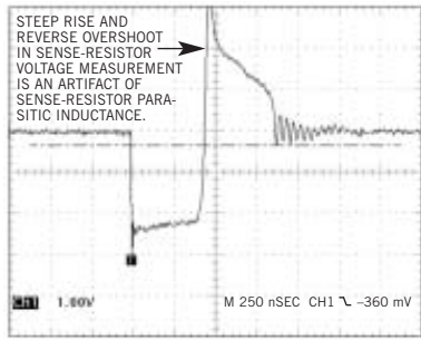
Figure 4 The steep rise and reverse overshoot in Figure 3's circuit are artifacts of sense-resistor parasitic inductance.
