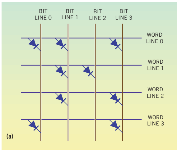
Figure 6 These 3-D-ROM thin-film diodes represent stored ones, and their absence reflects a zero (a). The addition of an antifuse makes the technology one-time programmable (b). Massively parallel accesses, coupled with 3-D stacking, help overcome the technology's slow random-read performance (c, courtesy 3D-ROM).
