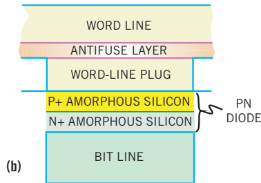
Figure 6 These 3-D-ROM thin-film diodes represent stored ones, and their absence reflects a zero (a). The addition of an antifuse makes the technology one-time programmable (b). Massively parallel accesses, coupled with 3-D stacking, help overcome the technology's slow random-read performance (c, courtesy 3D-ROM).
