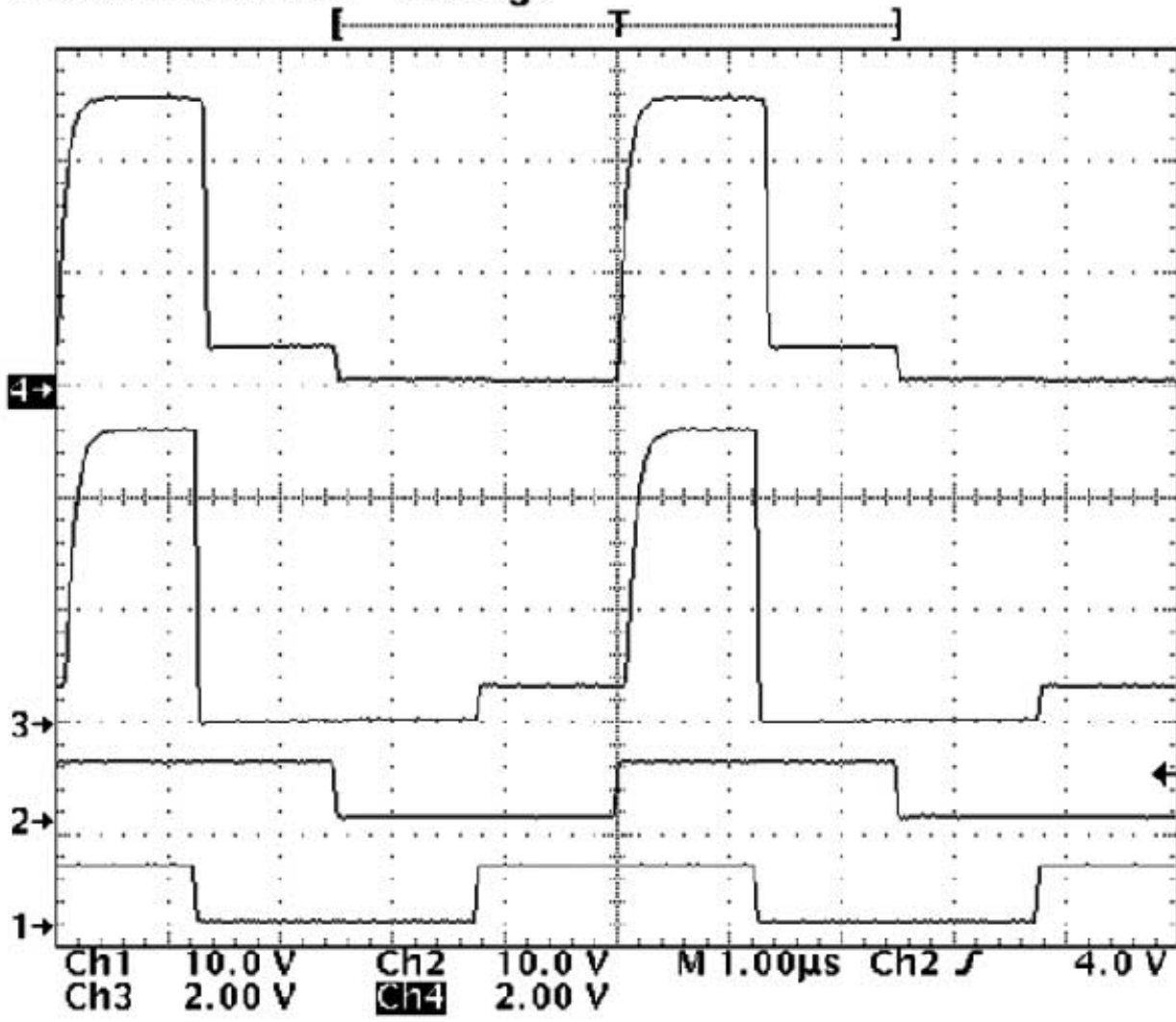
This scope photo shows the operation of the improved I 2 C isolator.
