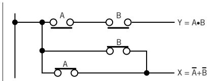
Figure 1 This circuit offers redundancy in machine-control applications.
