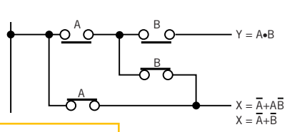
Figure 2 Boolean arithmetic proves that this circuit is equivalent to that of Figure 1.
