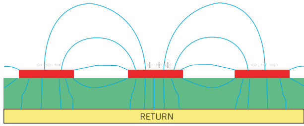
Figure 4 Electric-field distributions around three, closely coupled, 50\Omega microstrip traces in FR4 show the fringe fields changing with the bit patterns. Aggressor lines have the same bit pattern as the victim (a) and complementary bit patterns (b).
