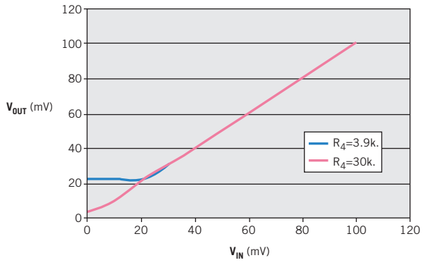
Figure 3 With 0.5-mA load current, the output voltage is linear down to 4 mV.
