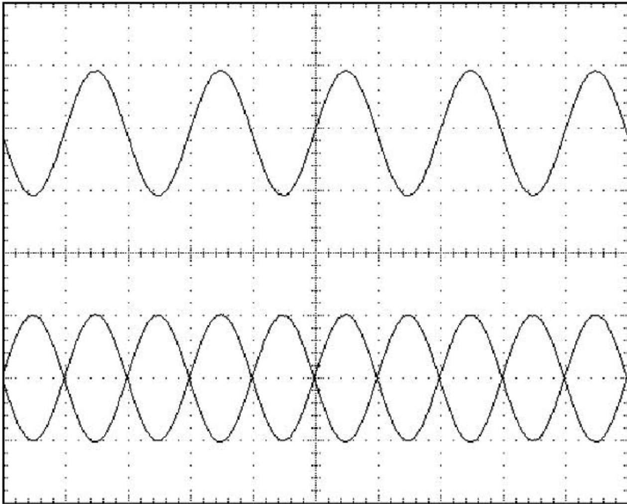
A 2V p-p, 1-kHz input signal (top), and 1V p-p differential-output signals (bottom) have an output common-mode voltage of 2.5V.
