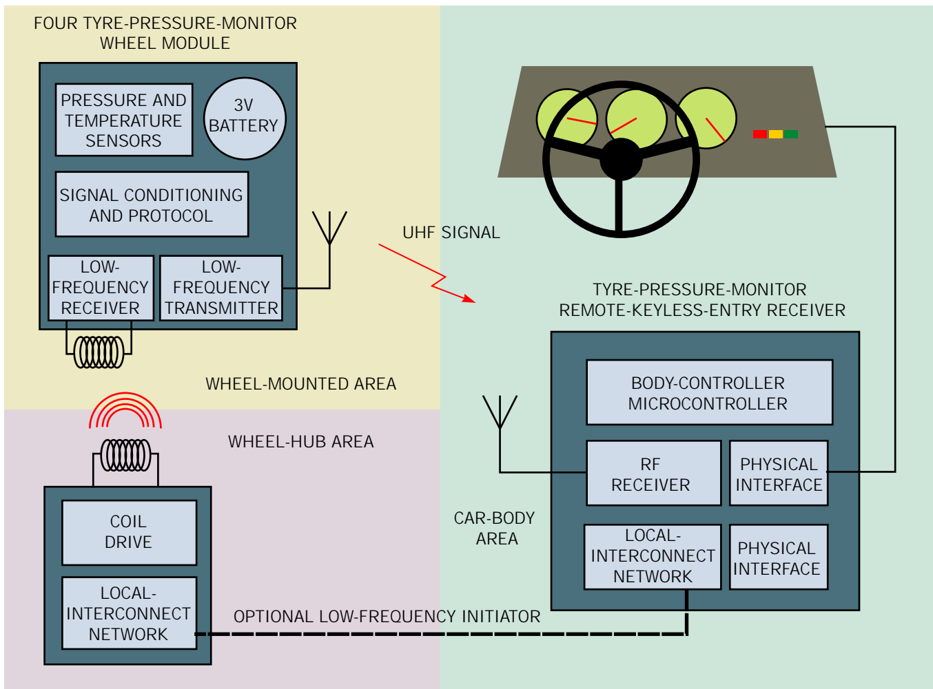
A typical direct-measurement system links wheel modules to a central receiver that interfaces with the vehicle's information bus, with an optional command channel providing duplex capability (courtesy Motorola).
