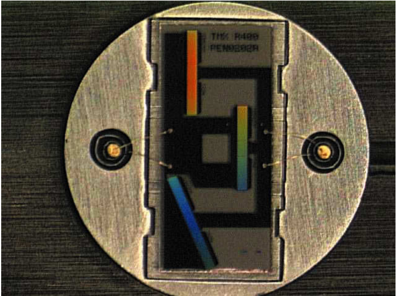
The spacing between fingers of interdigital transducers determines the wave period in a SAW device.
