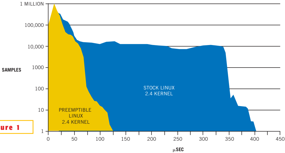
MontaVista Software's modified Linux kernel demonstrates dramatic improvements in pre-emption latency for the IBM PowerPC 440GP.
