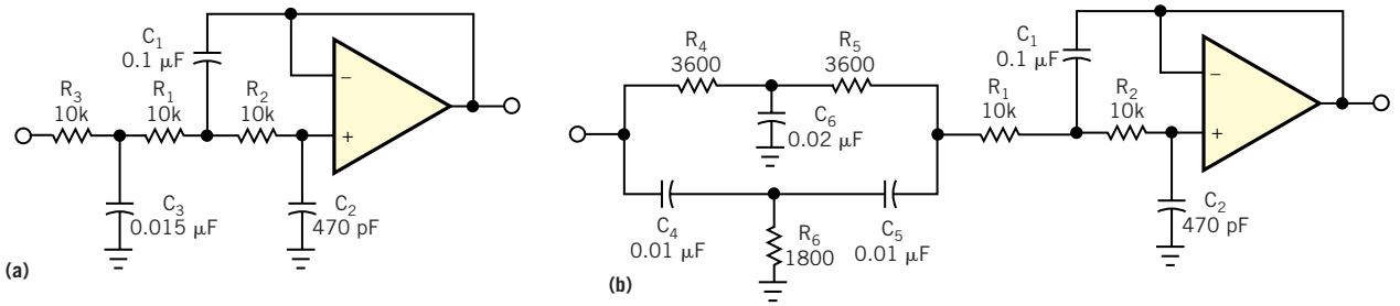
Figure 1 The addition of a twin-tee network (b) considerably improves the roll-off rate of the circuit (a).
