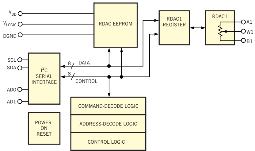
Figure 3 This block diagram shows the digital potentiometer's inner workings.
