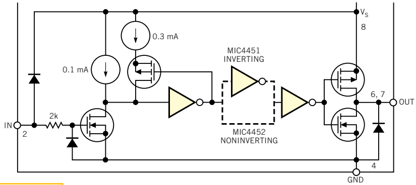
Figure 2 The MIC445x FET driver includes low-on-resistance complementary FETs.
