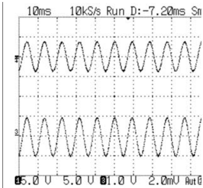
Figure 2 The sinusoidal input is 8V p-p (top trace), and output is 1800V p-p (bottom trace).
