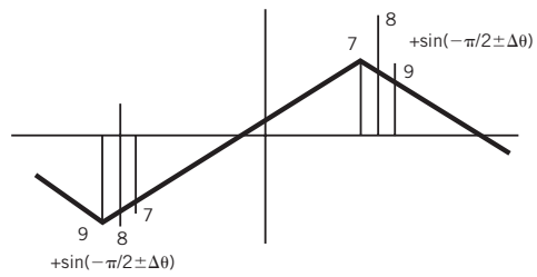
Figure 2 Signal detection (demodulation) involves sensing the points at which the phase of the RF carrier jumps from advanced to retarded or retarded to advanced (with respect to the phase of an unmodulated carrier). The decoder can then generate a triangular wave such as this one. (The time intervals labeled 7, 8, and 9 refer to the conditions of Figure 1.)
