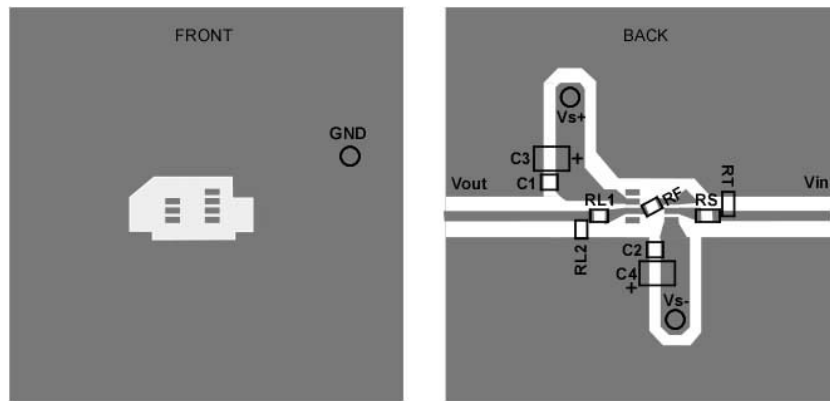
Figure 3 Back-side-power-supply runs require vias, which create incremental inductance.
