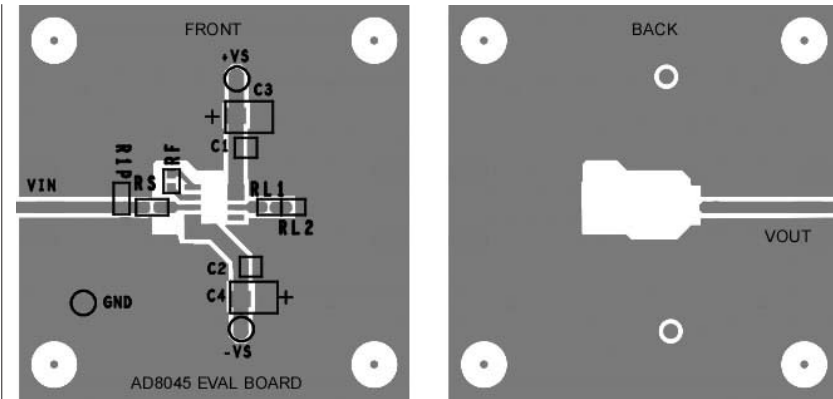
Figure 4 Front-side-power-supply runs don't increase distortion.
