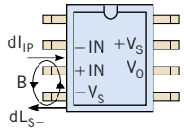
Figure 9 A standard SO-8 pinout results in mutual inductance coupling.
