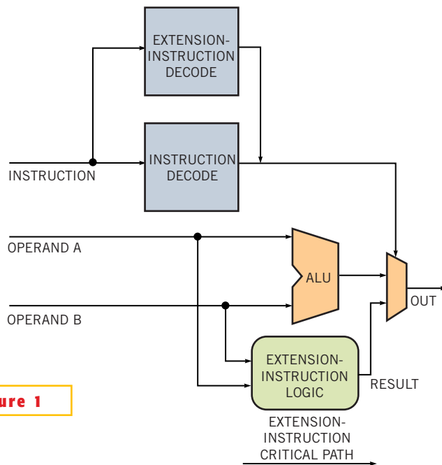
A custom instruction is an extension of the processor's ALU (arithmetic-logic unit) and instruction decoder. The custom instruction logic may be a critical path that can affect the processor clock rate unless you implement pipeline-stall controls or instruction pipelining.
