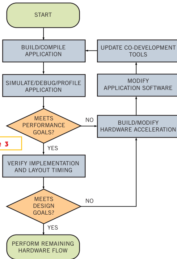
A generalized design flow for accelerating software highlights the performance-simulation and implementation-verification loops when building custom hardware acceleration.
