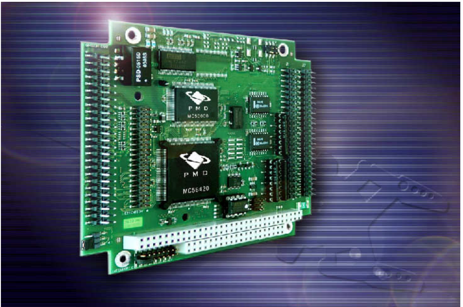
The Magellan-PC/104 card supports dc brushed, brushless dc, and stepper motors and communicates via a 16-bit parallel bus, CANbus, or serial port.
