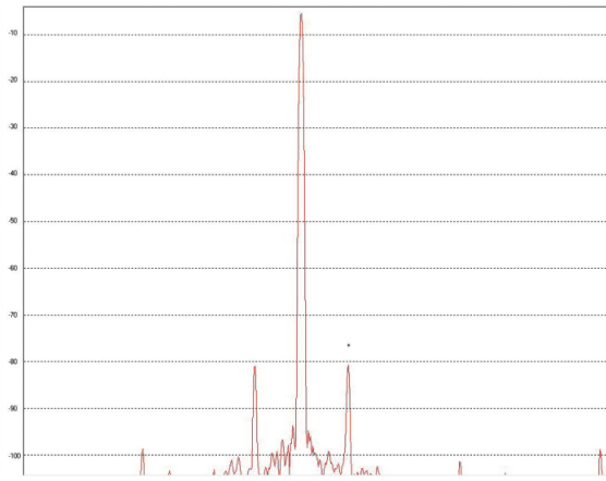
Figure 3 A phase-modulated encoding source from Figure 2 samples a 30.62-MHz pure sine source, resulting in a side-spur level of -74 dBc.
