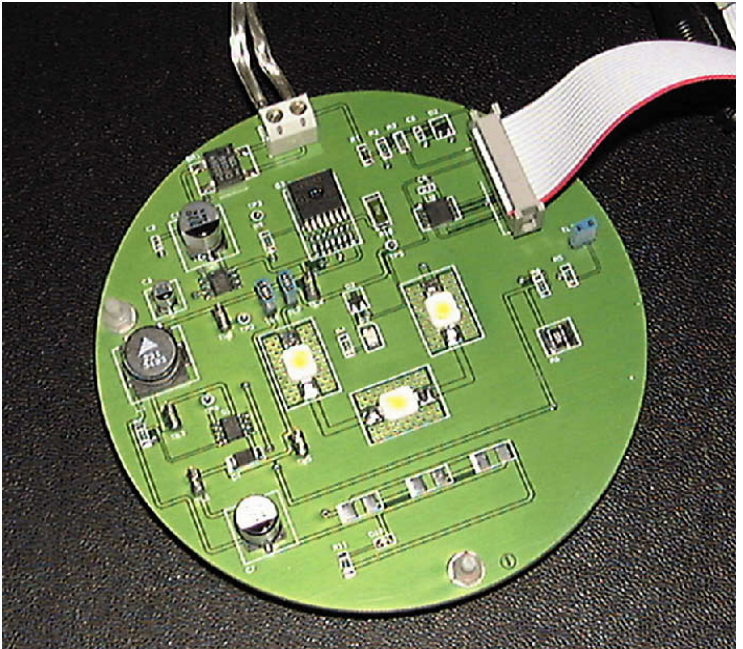
Careful design allows low-cost FR4 to dissipate several watts from multiple LEDs.
