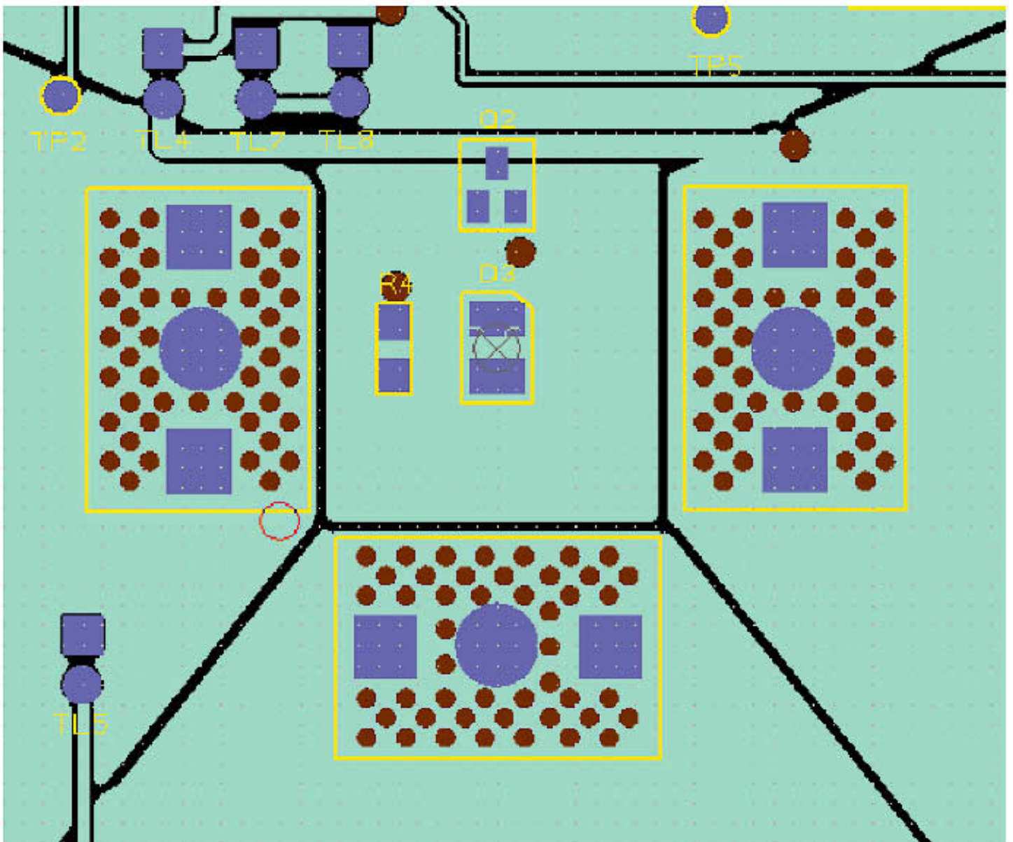
Thermal vias flow heat away from the LEDs and into surrounding solid copper areas.
