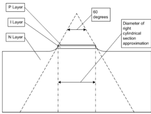
Figure B The mechanical cross-section leads to the right-cylindrical section approximation used for thermal analysis.
