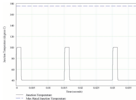
Figure E At a 10% duty cycle and burst width of 1.5 msec, junction temperature does not exceed 100°C for the sample parameters.
