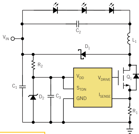
Figure 3 Zetex's ZXSC310 fits in a SOT-23-5 package and, in conjunction with an external pass element and a few other external components, make a compact controller/driver circuit for bright LEDs, replacing low-voltage halogen fixtures.
